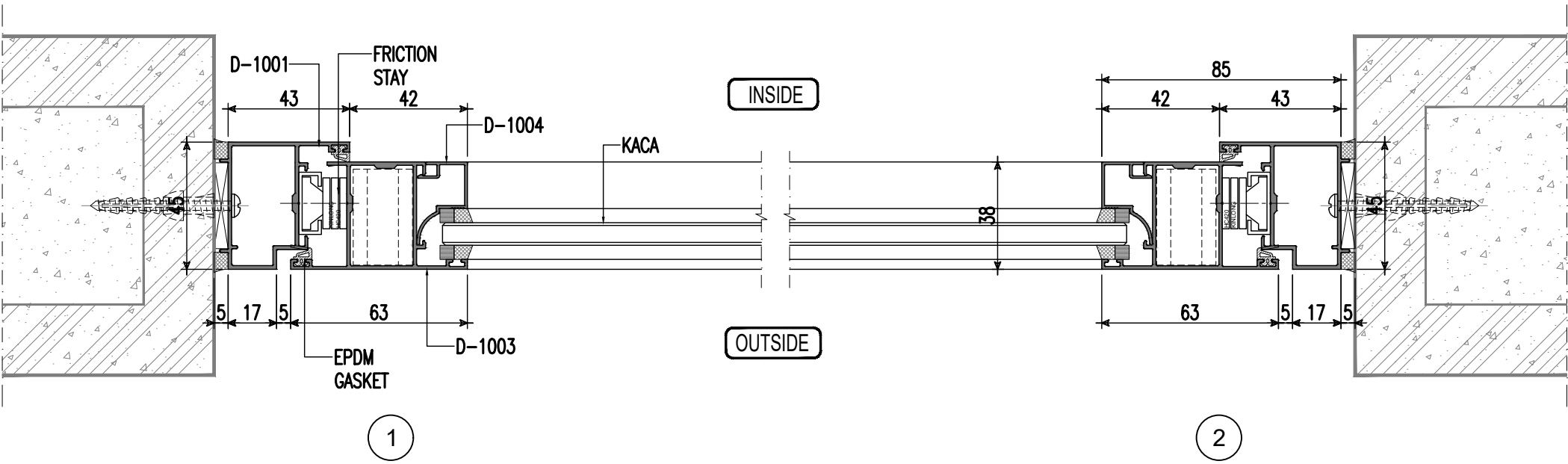
Detail Horizontal
