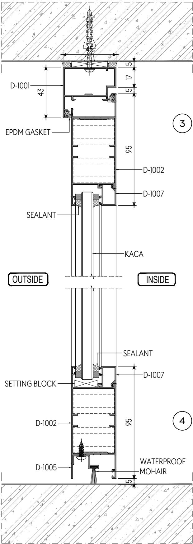
Detail Vertical
