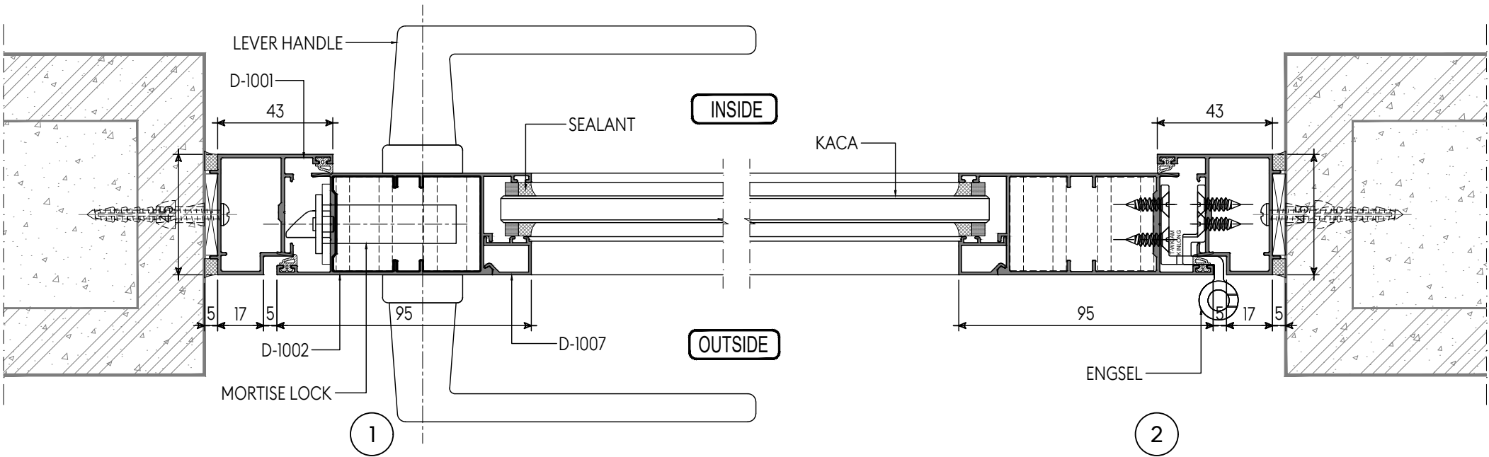
Detail Horizontal
