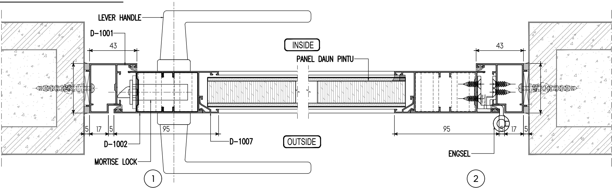
Detail Horizontal
