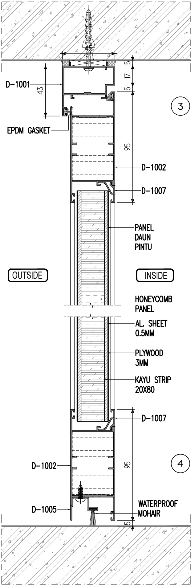
Detail Vertical
